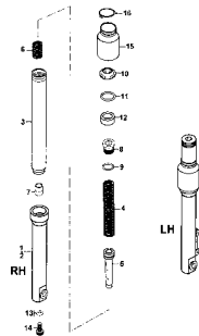
F22 Separated Parts Of Fr Fork
